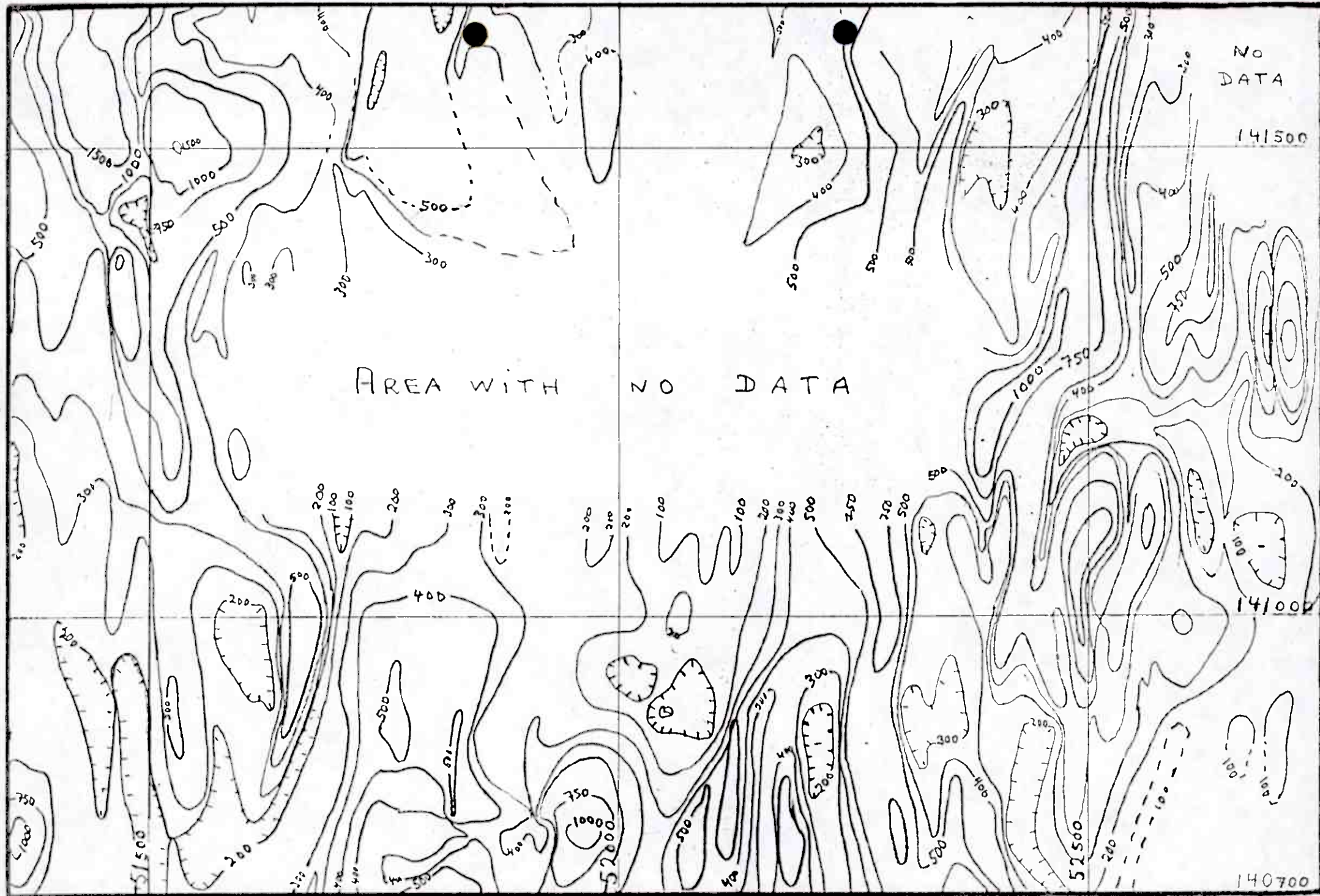
Fig. 4 Magnetic total field contour map redrawn from Carstens (1981).
