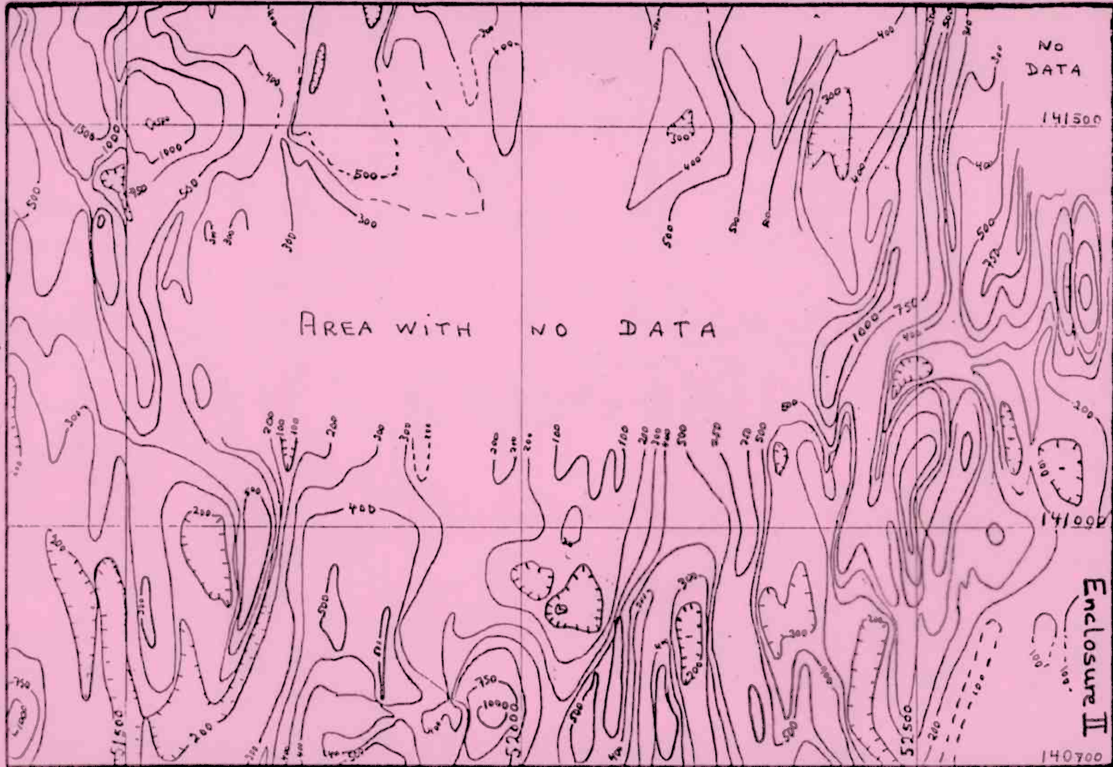
Magnetic total field contour map redrawn from Carstens (1981).
