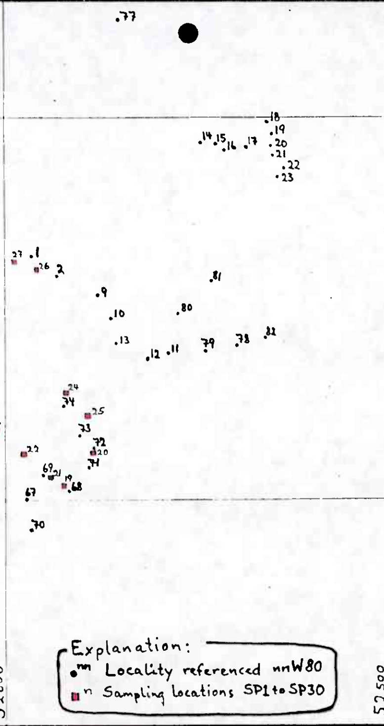
Fig. 3 Sample locations and localities referred to in field notes. VW 1980/81.
