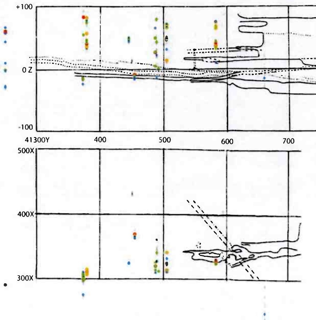
Figure 6: Vertical (Y-Z) and horizontal sections (Y-X) of the interval 41300-41750Y with the gold grades in drillholes displayed on a background of the old mine workings (yellow and red dots are >0.5 and >1 ppm Au, respectively, while green and blue are both <0.5 ppm). The horizontal section show the mine workings on level II.
