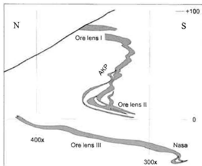
Figure 2: Schematic N-S profile from the westernmost part of the deposit, showing the general structure and division of the deposit into different ore lenses. The grid is 100 x 100 m.
