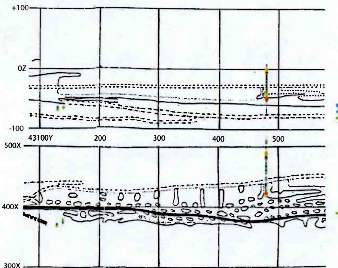
Figure 5: Vertical (Y-Z) and horizontal sections (Y-X) of the interval 43100-43600Y with the gold grades in drillholes displayed on a background of the old mine workings (yellow and red dots are >0.5 and >1 ppm Au, respectively, while green and blue are both <0.5 ppm).
