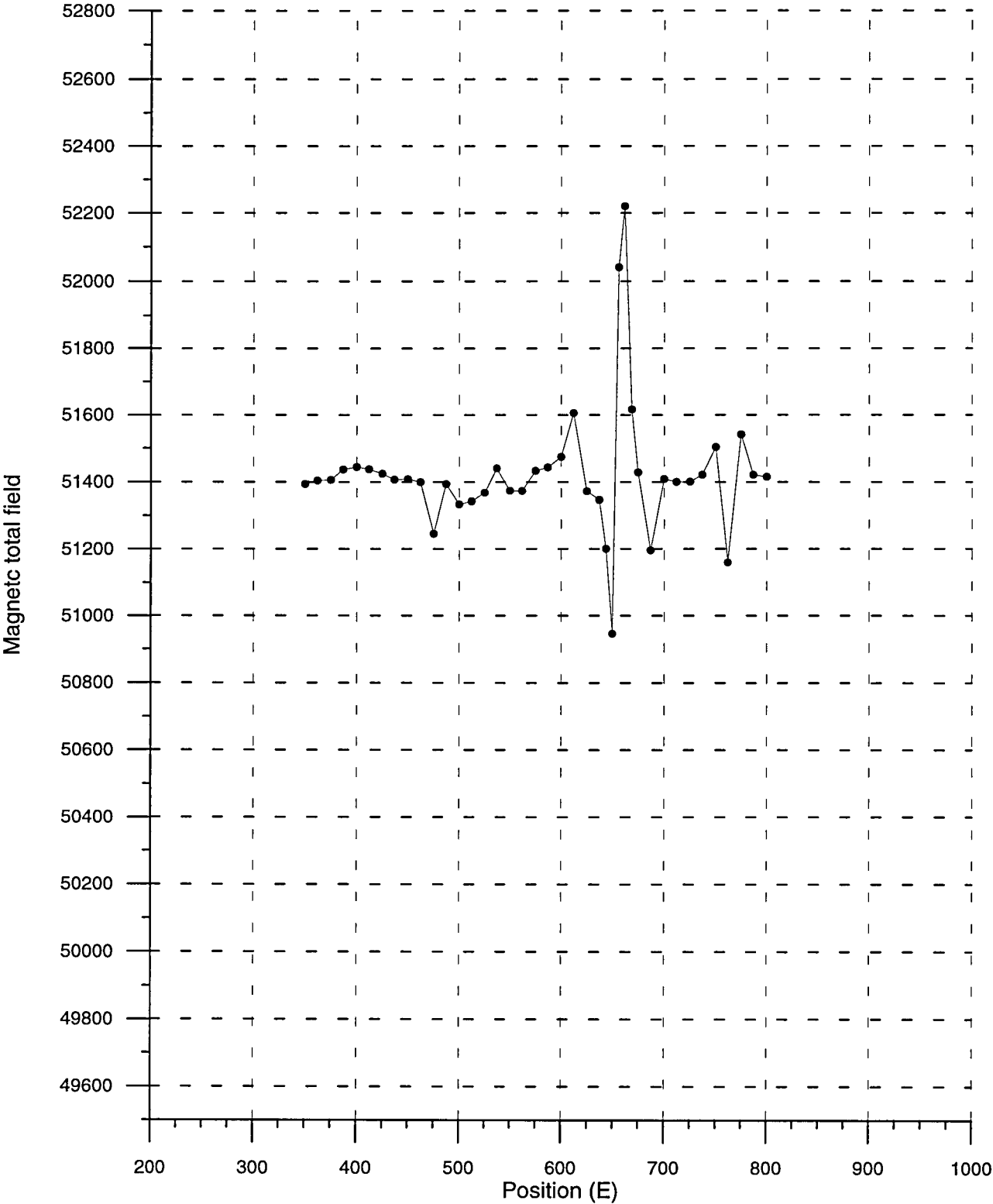
Figure 9. Magnetic total field profile 1100 N.
