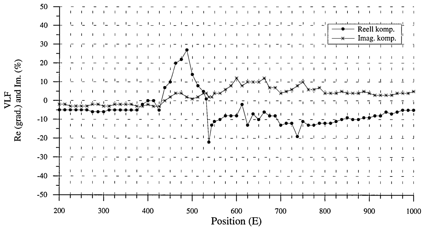
Figure 21. VLF profile 1100 N and 1150 N.
