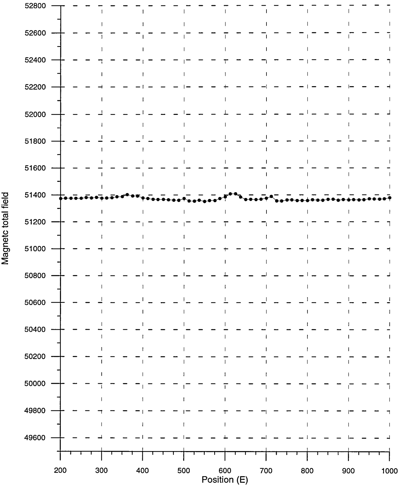
Figure 16. Magnetic total field profile 1450 N.
