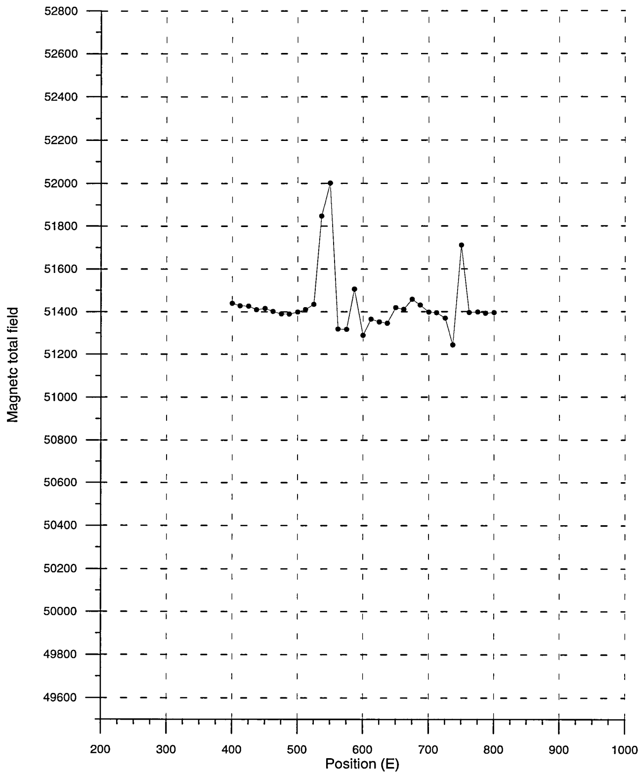
Figure 7. Magnetic total field profile 1000 N.
