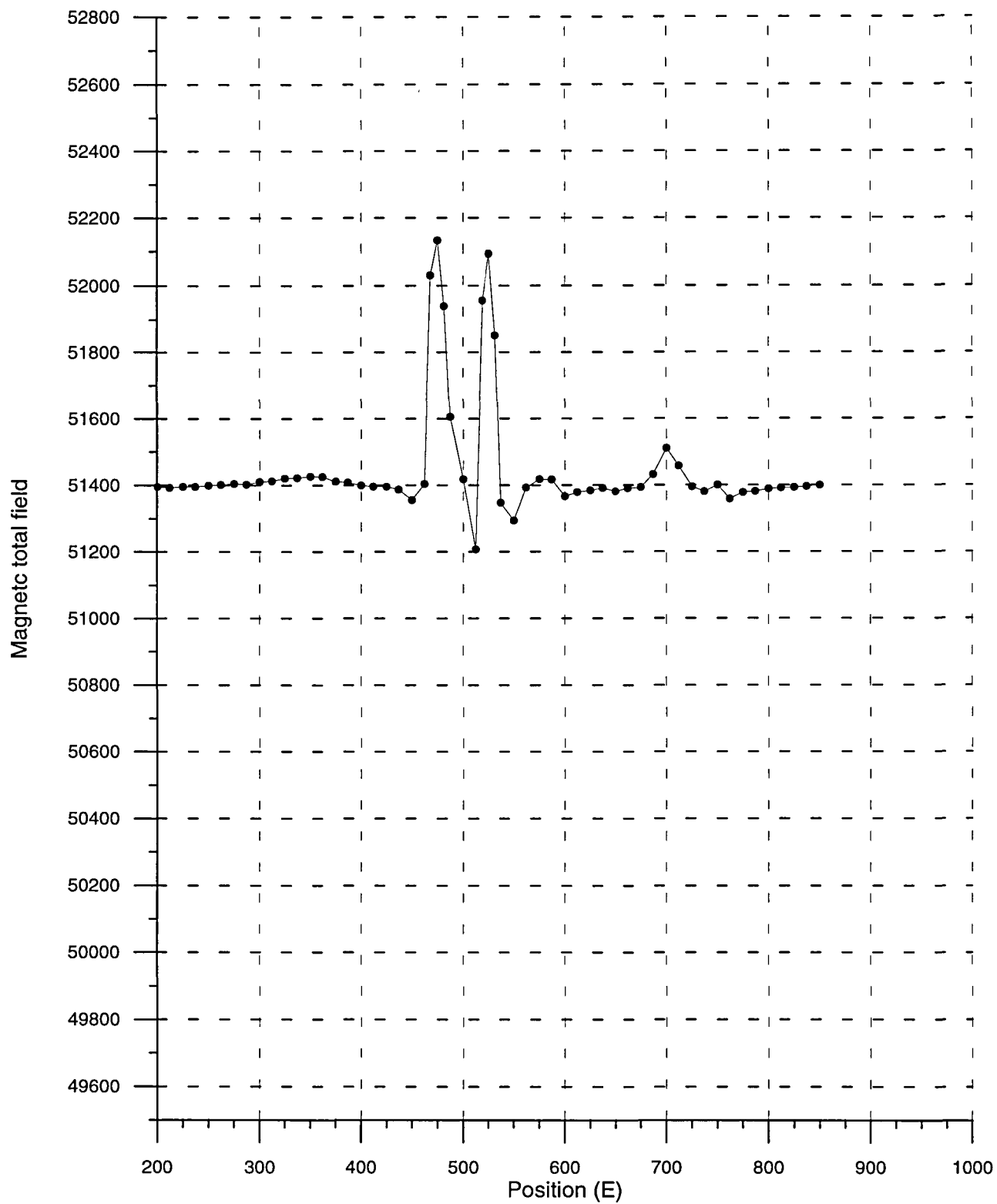
Figure 14. Magnetic total field profile 1350 N.
