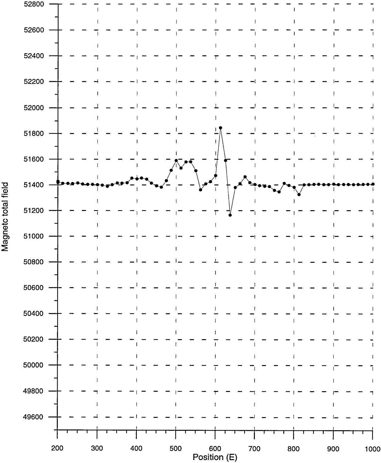
Figure 10. Magnetic total field profile 1150 N.
