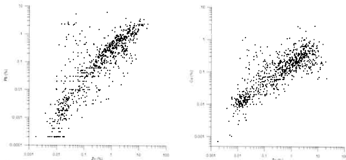
Figure 7: Lead (Pb) and copper (Cu) versus zinc (Zn) in intervals analysed on precious metals, all data. Note tails of high Pb and Cu values with low Zn values. Logarithmic scales.
