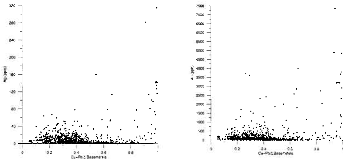
Figure 9: Silver and gold versus the ratio \text{Cu}+\text{Pb}/\Sigma \text{ base metals} .
