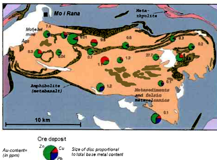
Figure 2: Overview of geology in the Mofjellet district with the major sulphide deposits displayed by discs with proportions of Zn, Pb, Cu. Numbers show highest gold values recorded in each deposit.
