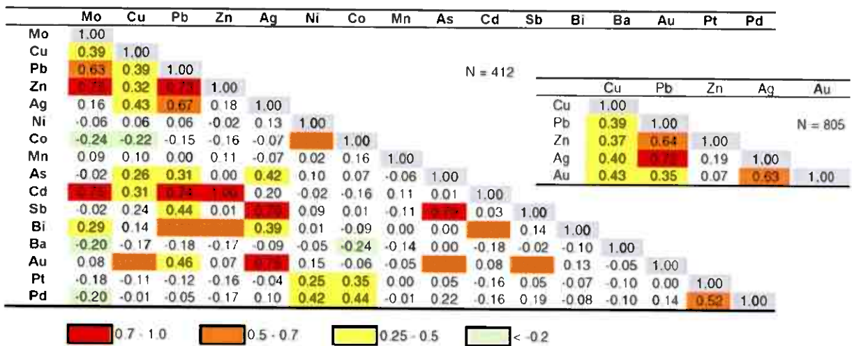
Figure 6a: Correlation matrix for the samples analysed by ACME laboratories. Coloured spaces show significant correlations between elements. The small matrix (b) includes the old data sets (from Kruse and Burman 1987).
