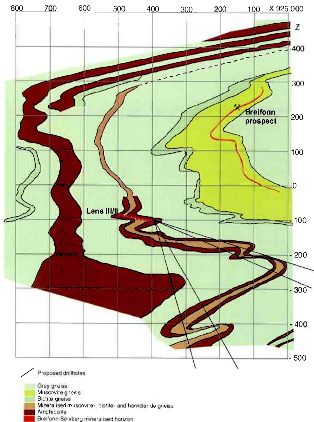
Figure 12. Geological profile of the Moffellet ore-bearing structure constructed from surface mapping. Grid refers to drill section in profile Y 44.800.
