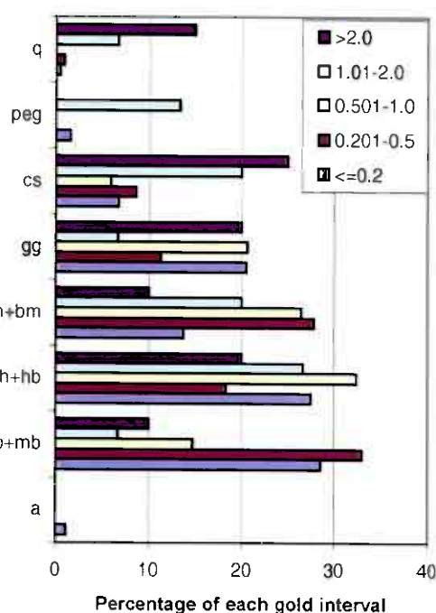
Figure 5b: Graph showing percentage of each interval of gold content that is found in the different lithologies.
