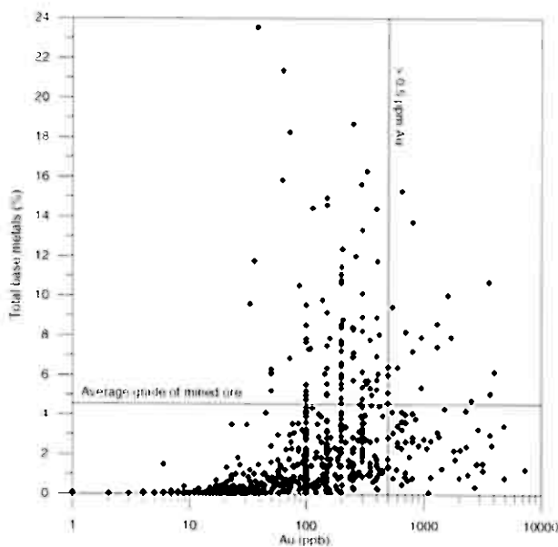
Figure 11: Total base metal content versus gold content, showing that gold is concentrated in zones with lower base metal contents.
