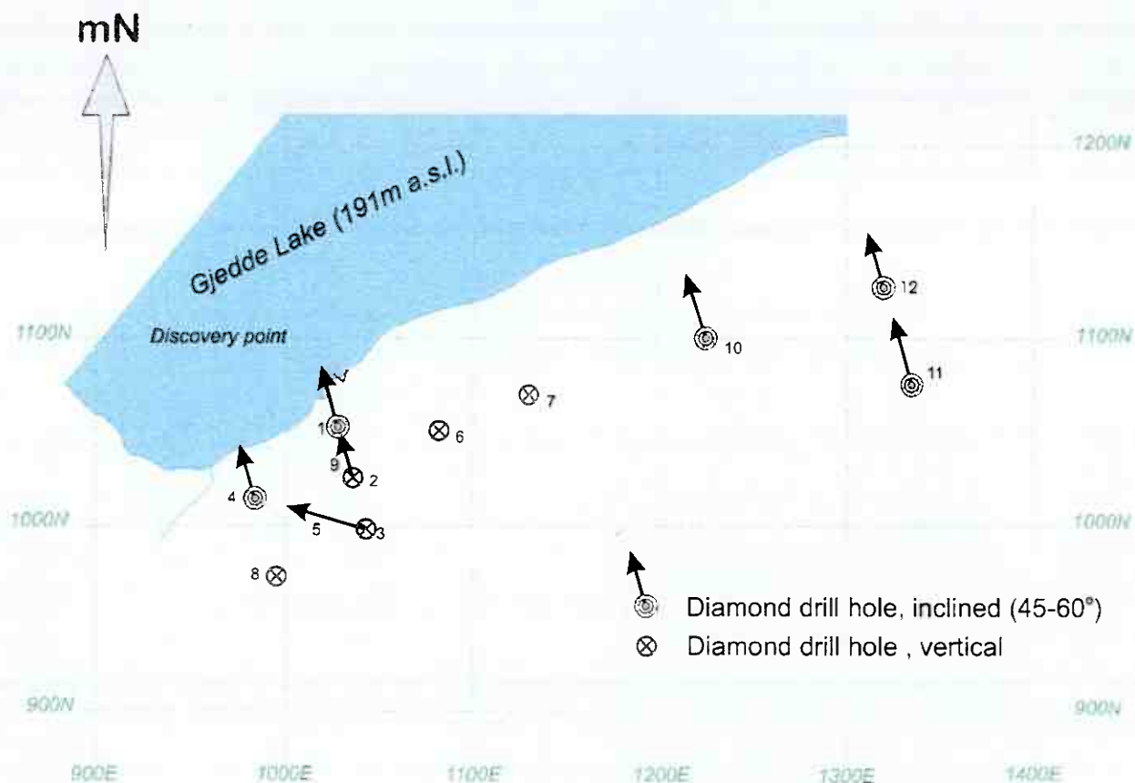
Fig. 2. Map showing the distribution of drill holes along the southern shore of Gjedde Lake. The inclined holes are drawn as horizontal projections. The grid lines are parallel to magnetic north.
