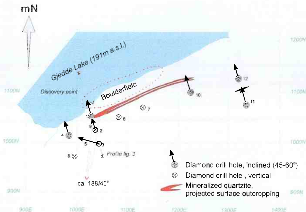
Fig. 7. Map showing the distribution of ice-transported auriferous BBQ-blocks in comparison to the extrapolated, blind outcrop of the BBQ at the 191 level (water).
