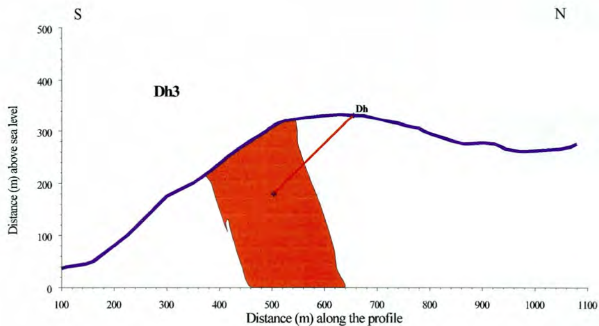
Fig.5c: N-S profile showing Dh3 and an estimation of the massive \text{TiO}_2 -rich eclogite (red). The direction of Dh3 is \text{N}100^\circ/45^\circ dip.
