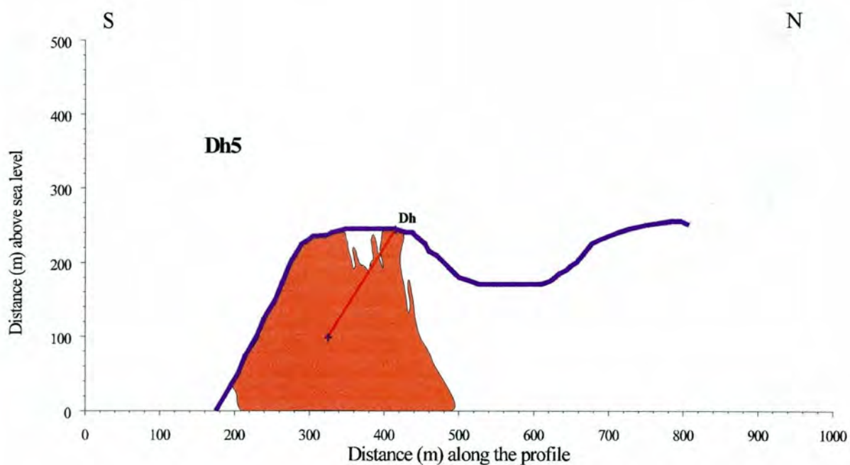
Fig.5e: N-S profile showing Dh5 and an estimation of the massive \text{TiO}_2 -rich eclogite (red). The direction of Dh3 is \text{N}90^\circ/60^\circ dip.
