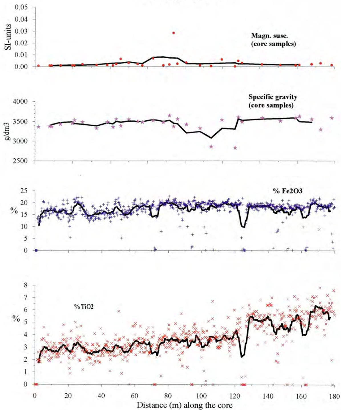
Fig. 13. Graph showing the variations in TiO 2 , Fe 2 O 3 , magn. susc. and specific gravity along Dh 5.
