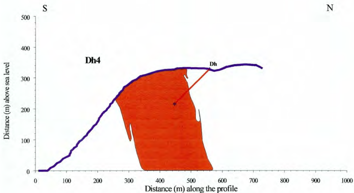
Fig.5d: N-S profile showing Dh4 and an estimation of the massive \text{TiO}_2 -rich eclogite (red). The direction of Dh3 is \text{N}100^\circ/45^\circ dip.
