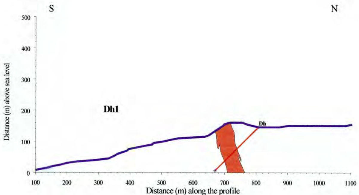
Fig. 5a: N-S profile showing Dh1 and an estimation of the massive \text{TiO}_2 -rich eclogite (red). The direction of Dh1 is \text{N}80^{\circ}/45^{\circ} dip ( \text{N}80^{\circ} refer to 80^{\circ} from N clockwise).
