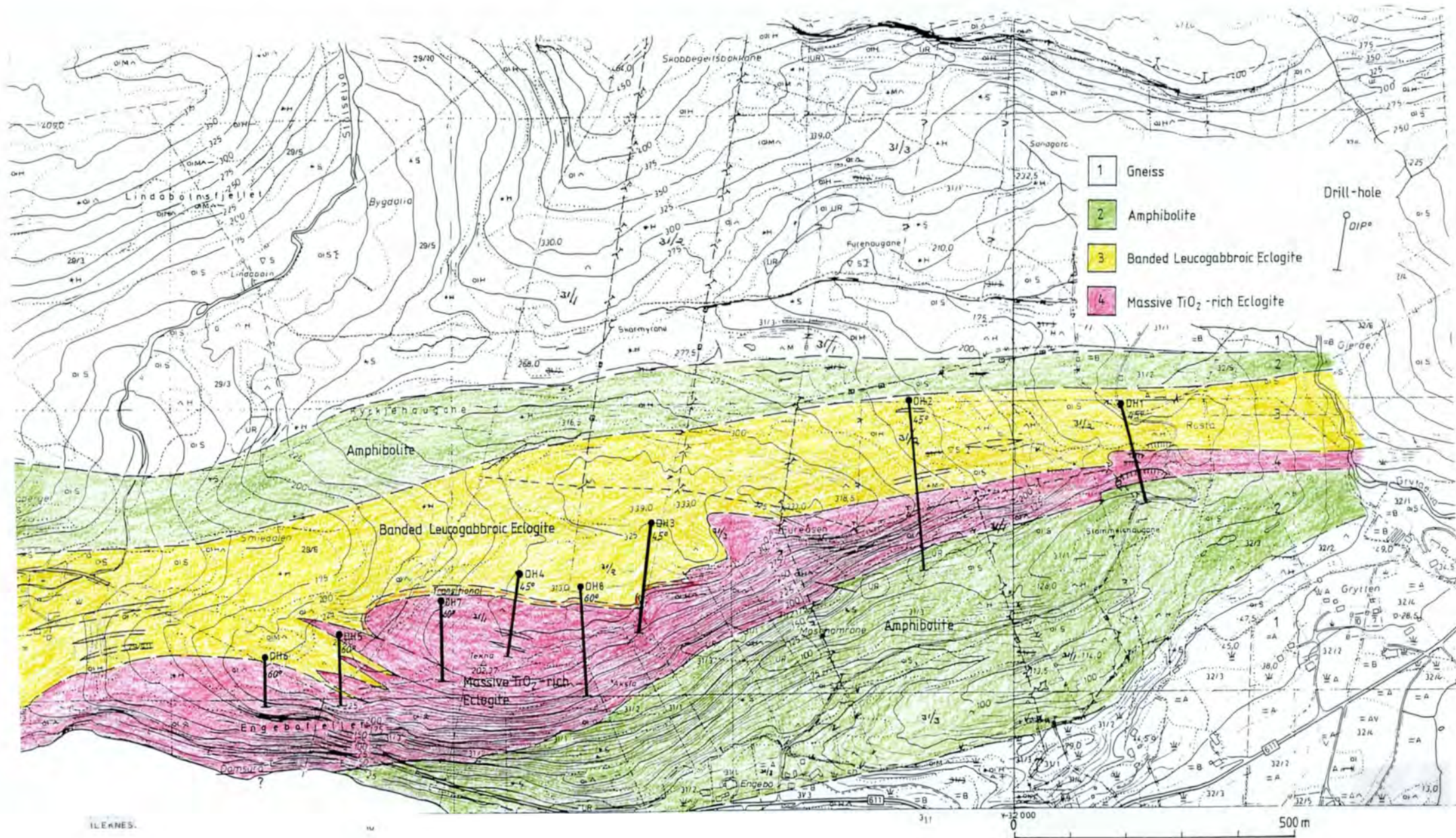
2: Simplified geologic map of the Engebøfjellet eclogite deposit (by Magnus Garson) with drill-hole locations. The directions of the drill-holes are: \text{N}80^\circ/45^\circ dip for Dh1 and Dh2, \text{N}100^\circ/45^\circ dip for Dh3 and Dh4, and \text{N}90^\circ/60^\circ dip for Dh5, 6, 7 and 8. N-S vertical profile sketches of Dh1 to 5 are shown in Fig. 5.
