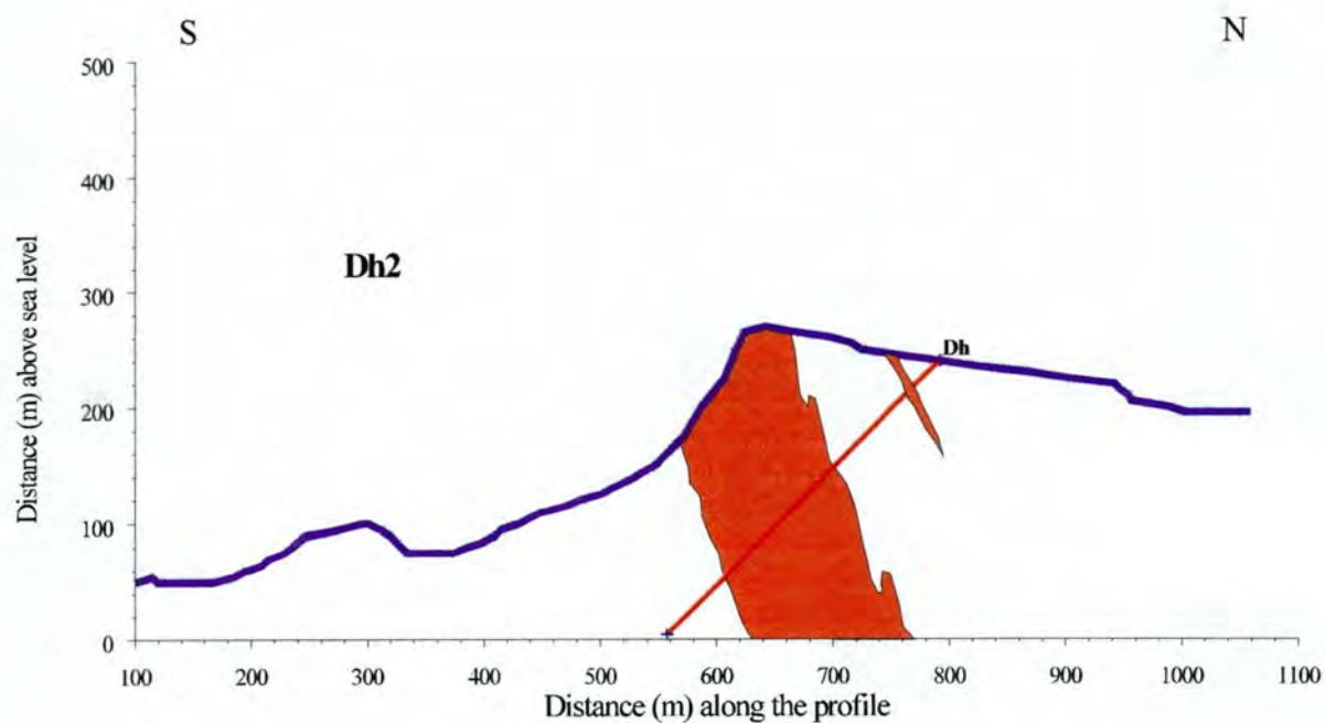
Fig.5b: N-S profile showing Dh2 and an estimation of the massive \text{TiO}_2 -rich eclogite (red). The direction of Dh2 is \text{N}80^\circ/45^\circ dip.
