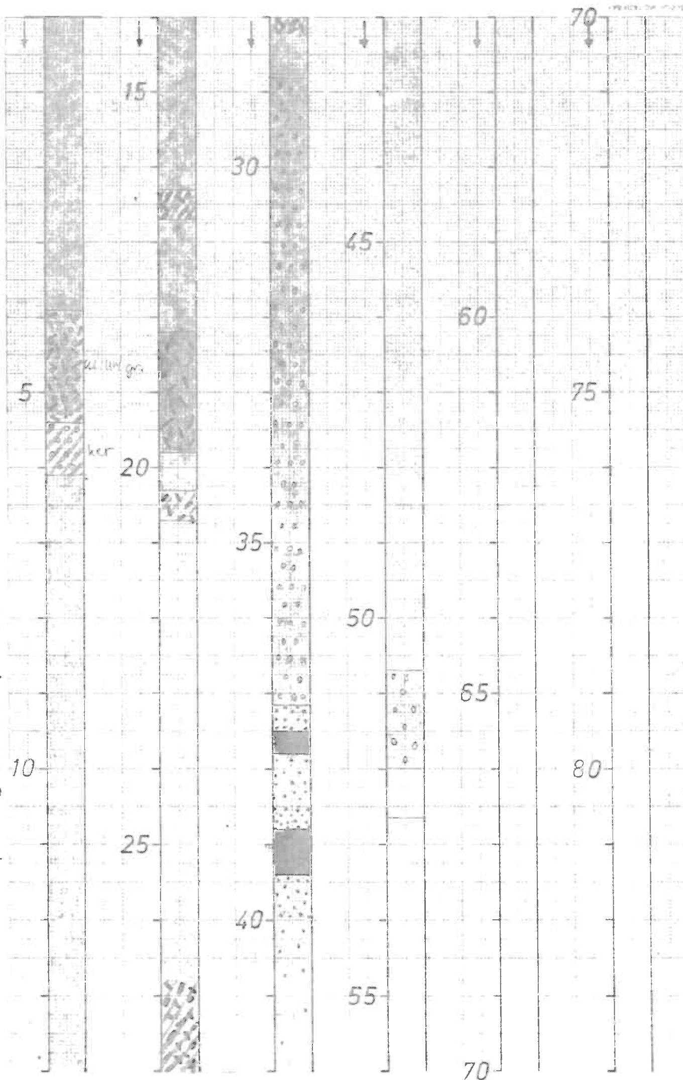
The petrographical profile of the borehole nr.181, Grimsdalen.
