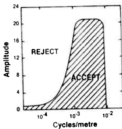
Frequency response of magnetic operator
