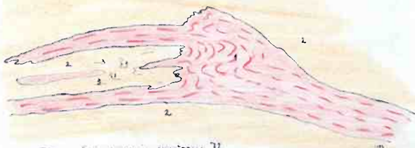
Fig 3 Skisse inn i skistross 72
