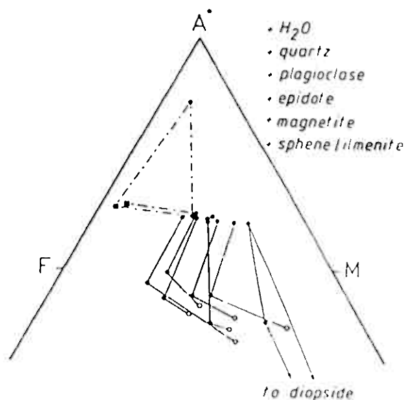
Figure 10 A*-F-M plot of amphibolite facies assemblages in intermediate to basic rocks. Squares = garnet, other symbols as on Fig. 9.
