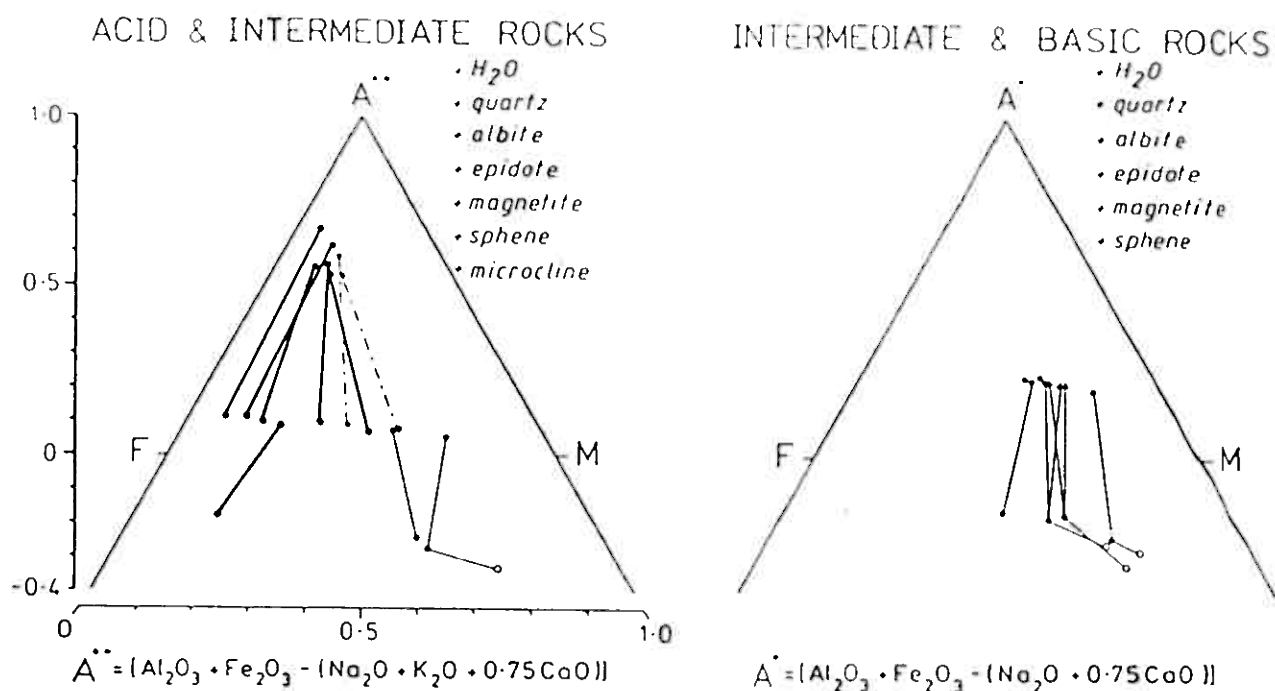
Figure 9 A*-F-M and A*-F-M projections for albite bearing rocks from the Rombak window. K-white micas plot at the top of the diagram, biotites and chlorites (triangles) in the centre and amphibole at the bottom. Open circles indicate amphibole cores. K-white micas, biotite and chlorites represent the average of several analyses, but the range is smaller than the symbol used. Heavy lines = granites, light lines = intermediate and basic rocks, dashed lines = sheared intermediate and basic rocks.
