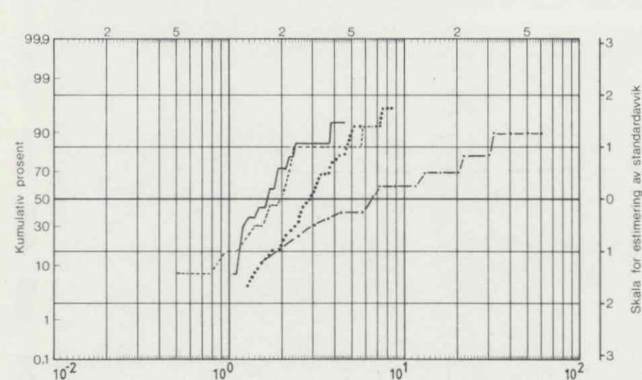
FREKVENSFORDELINGS-DIAGRAM FOR Th/K
