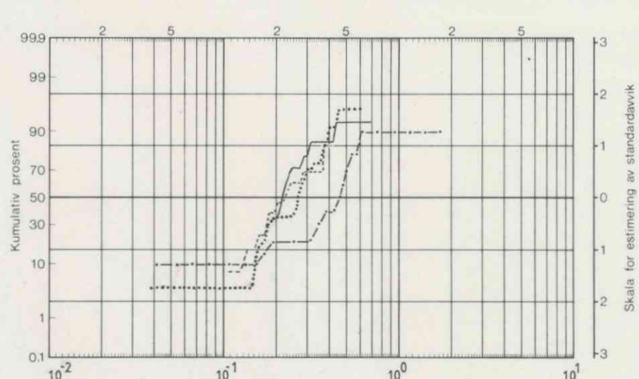
FREKVENSFORDELINGS-DIAGRAM FOR U/K
