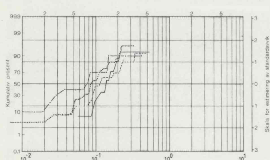
FREKVENSFORDELINGS-DIAGRAM FOR U/Th
