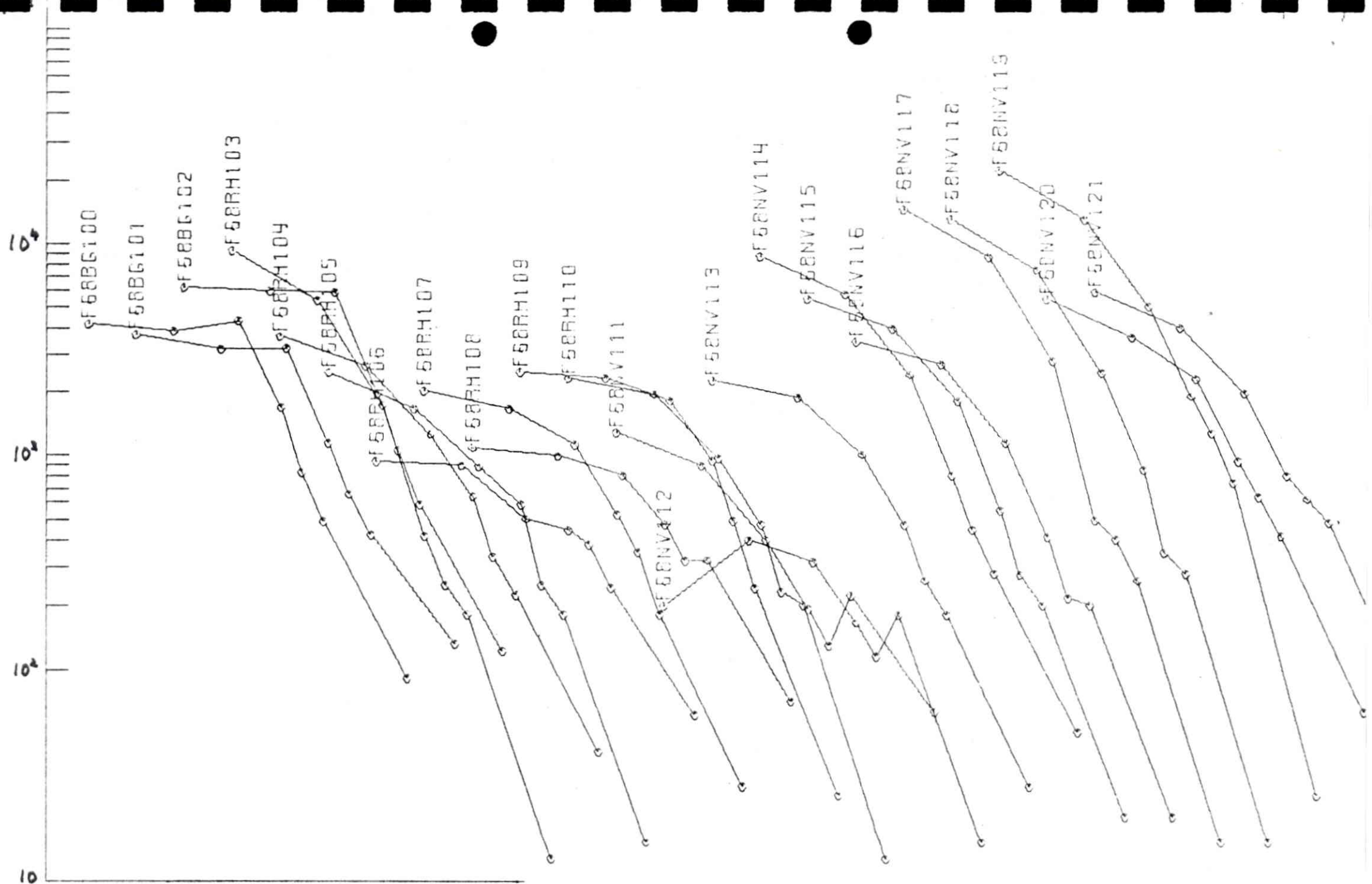
Fig. 4 Chondrite-normalized REE spectral diagrams for Fe-rich rocks
